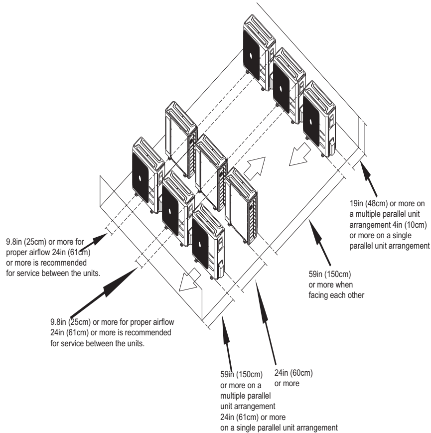
Fig. 9 — Clearances for multiple units
