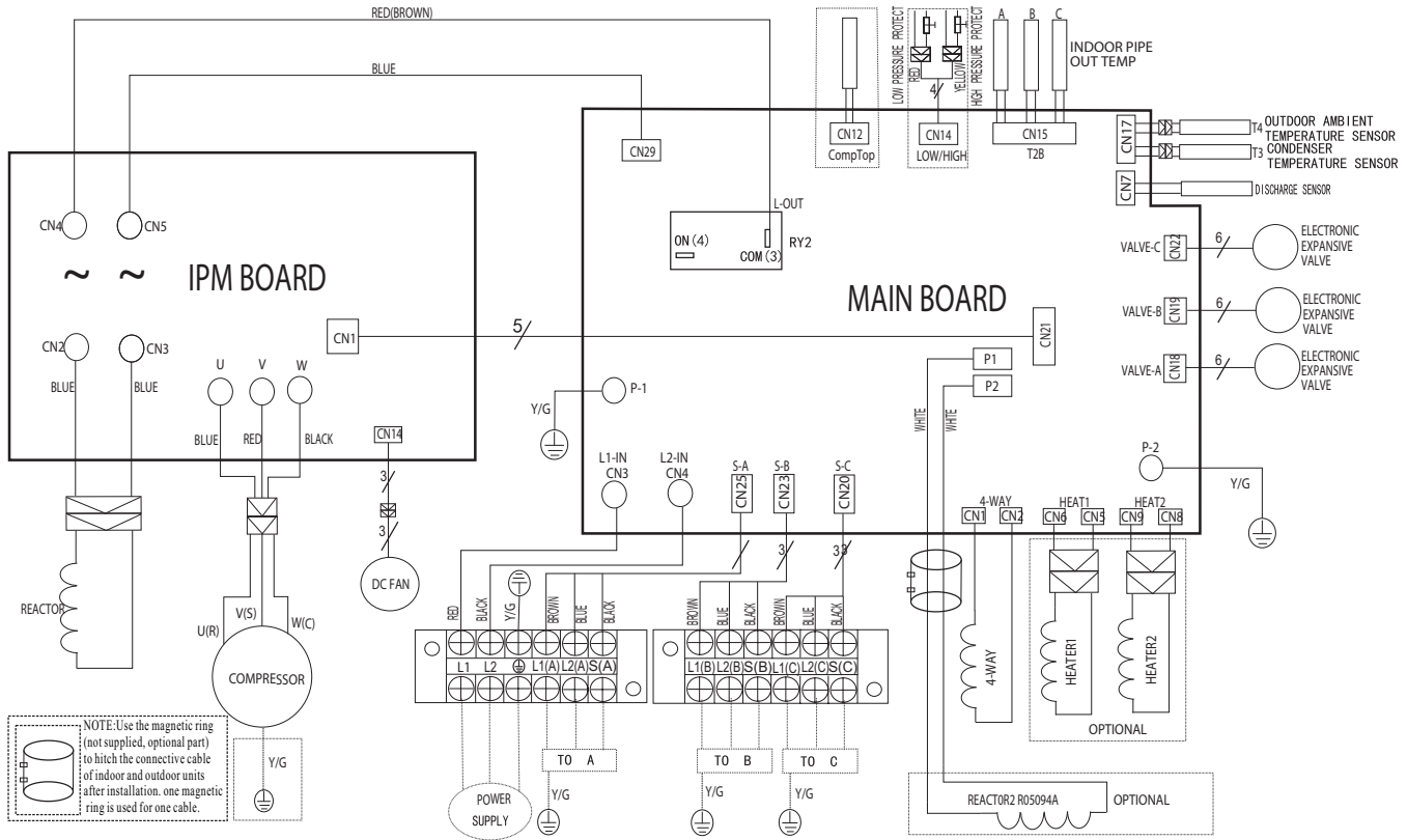
Fig. 12 — Wiring Diagram 27K - 3 Zone Max
