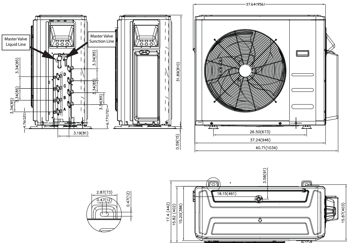
Fig. 6 — Outdoor Dimensions Size 36K
