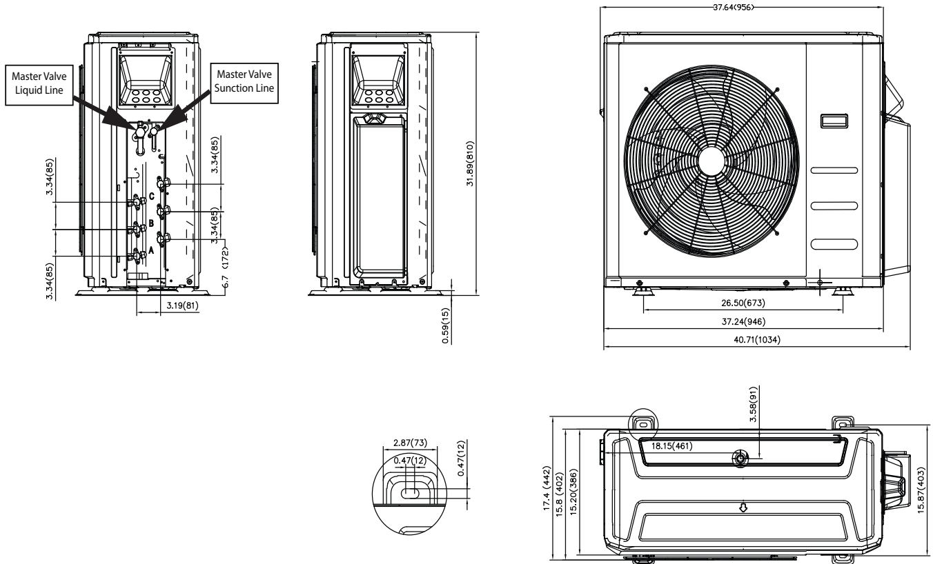
Fig. 5 — Outdoor Dimensions Size 27K
