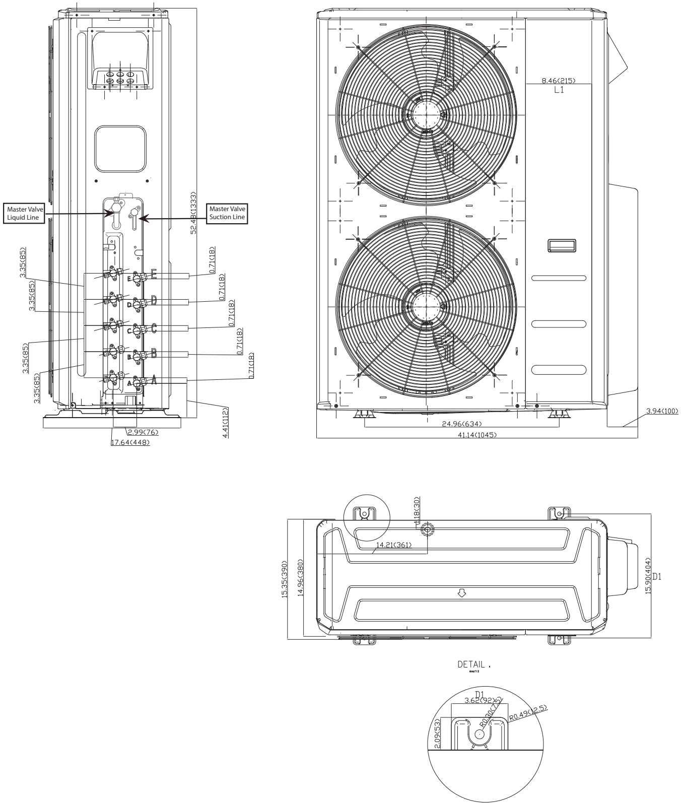
Fig. 7 — Outdoor Dimensions Size 48K
