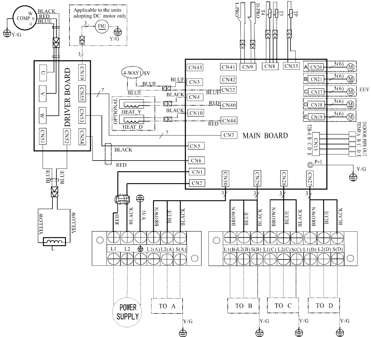
Fig. 13 — Wiring Diagram 36K - 4 Zone Max
