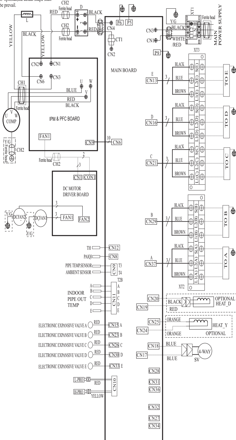
Fig. 14 — Wiring Diagram 48K - 5 Zone Max
